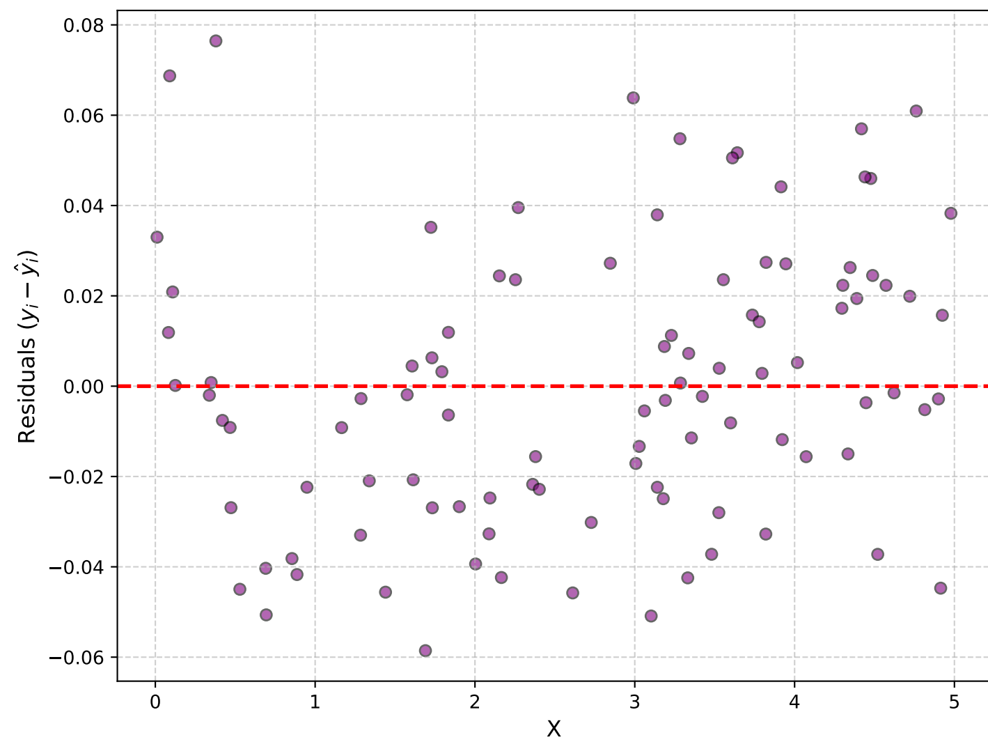
Residual Plot
